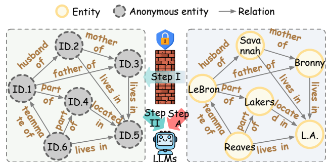
Figure 1: Comparison between previous RAG (Step A) with privacy-protected RAG (Step I-II) system for KGQA.
